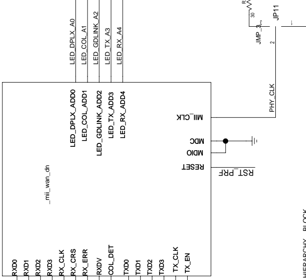
MII ETHERNET HIERARCHY BLOCK PAGES 26-27
